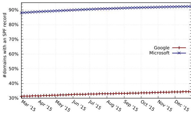
Fig. 5. SPF usage growth for cloud e-mail providers in the .com TLD.
