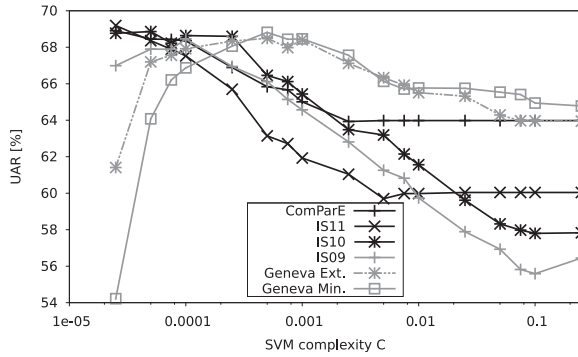
Fig. 1. Individual results (UAR [%] versus SVM complexity—all 17 values, see Section 4.3) for the TUM-AVIC database (categories: three levels of interest).
